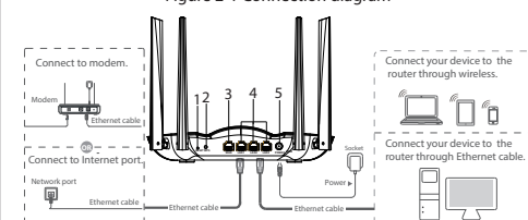
Figure 2-1 Connection diagram
